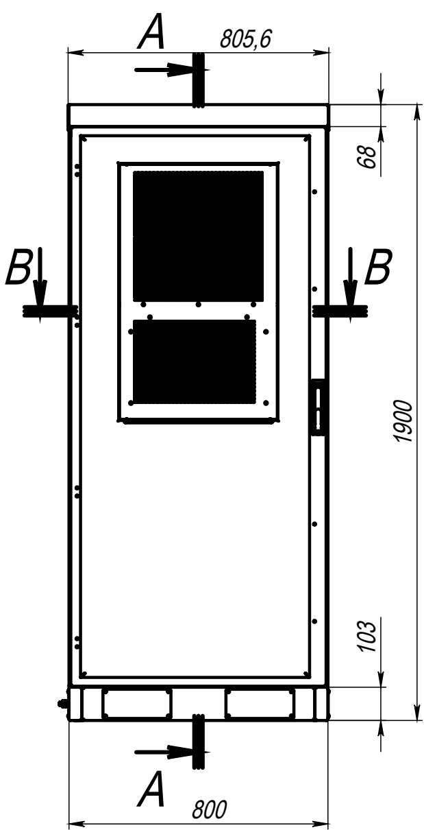
Dimensional drawing: Outdoor cabinet B36
