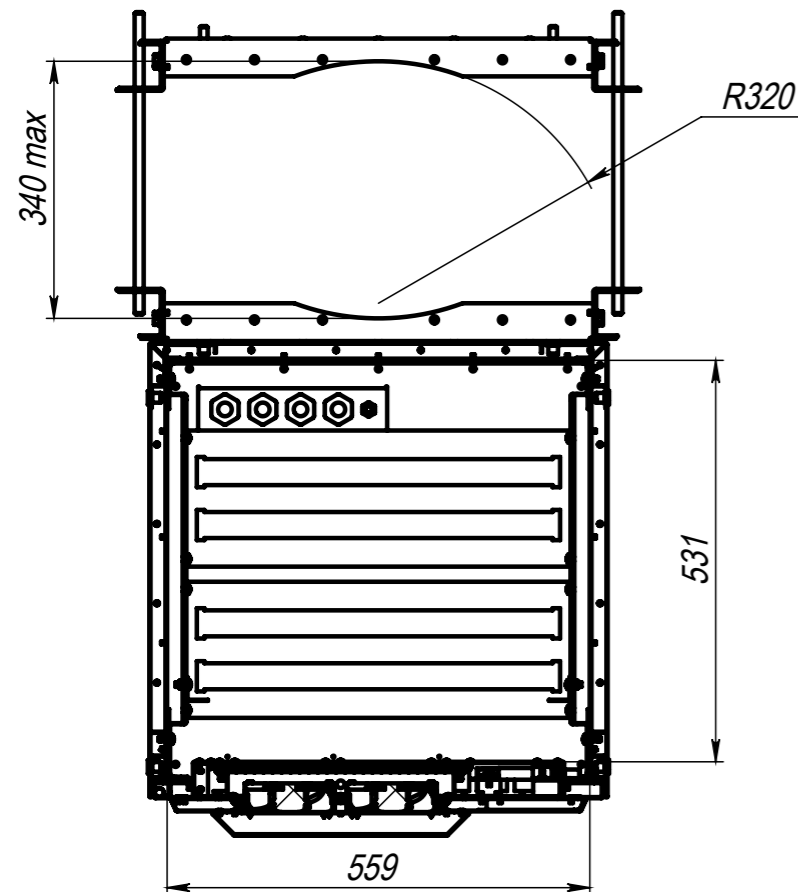
B-B Internal dimensions
