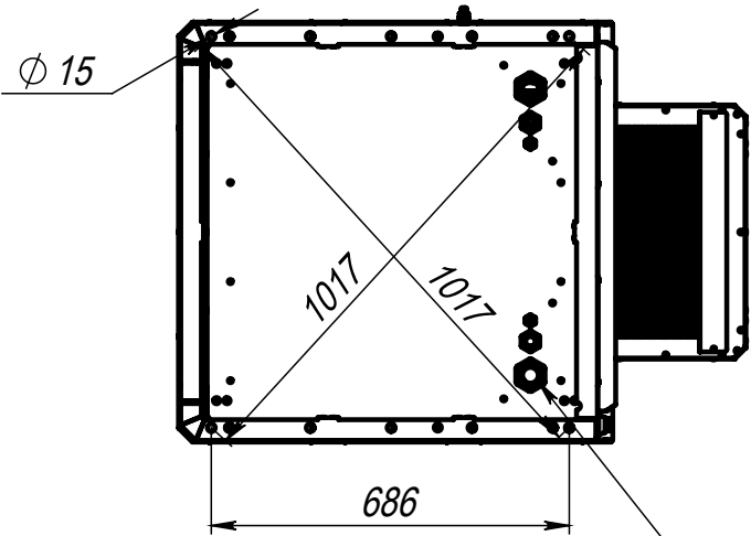
Mounting holes
