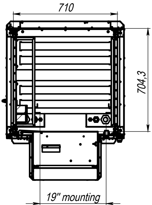
B-B Internal dimensions
