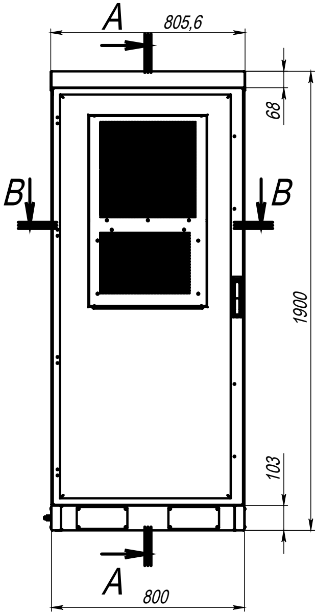
Dimensional drawing: Outdoor cabinet T36
